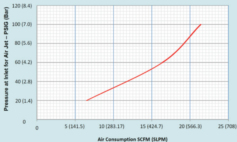
Air Consumption at various Pressures for Air Jet Model 45002/45002B/ 45002S - 0.008" Gap Setting
