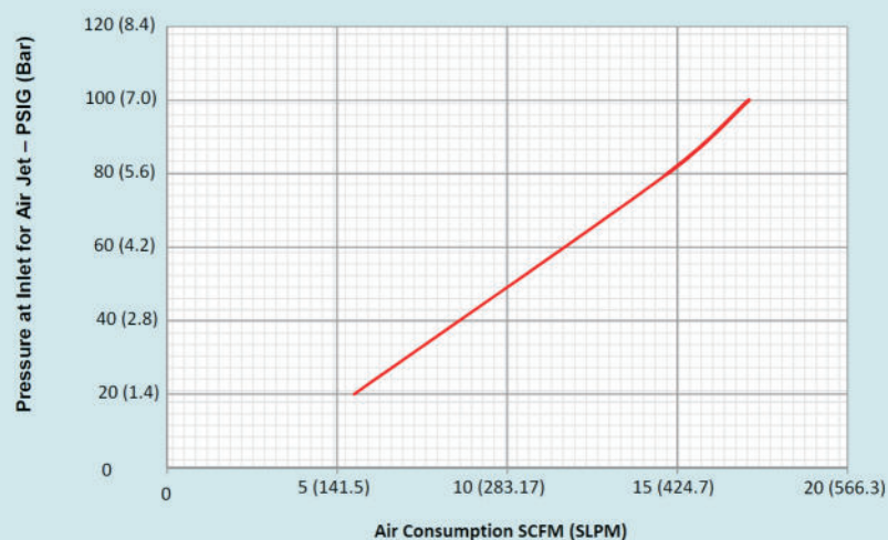
Air Consumption at various Pressures for Air Jet Model 45001 – 0.008" Gap Setting
