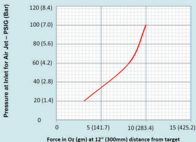
Force at various Pressures for Air Jet Model 45001 – 0.008" Gap Setting
