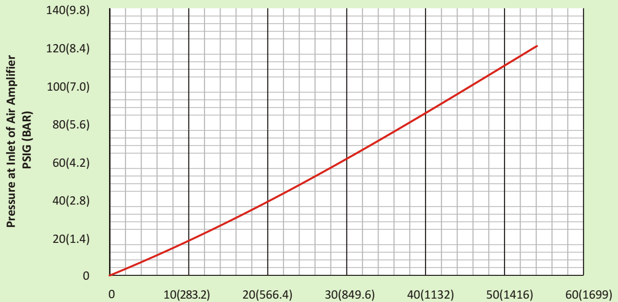
Pressure vs. Air Flow At Outlet for Model AM 10 Standard Air Amplifier
