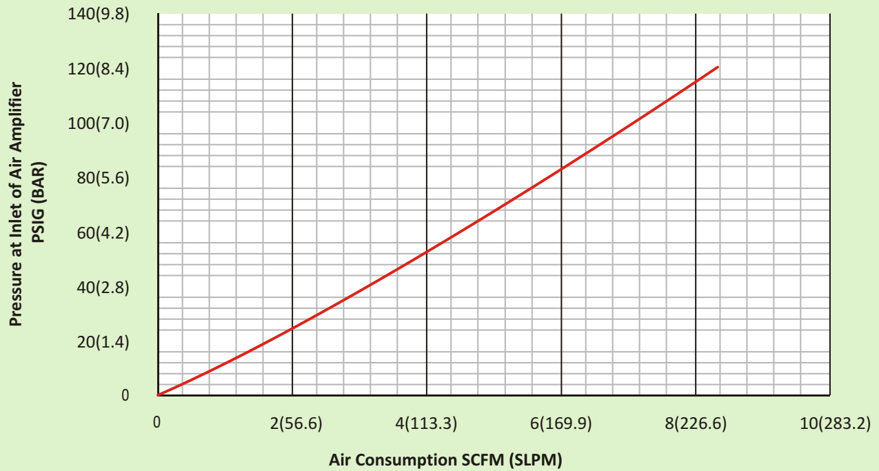
Pressure vs. Air Consumption for Model AM 10 Standard Air Amplifier
